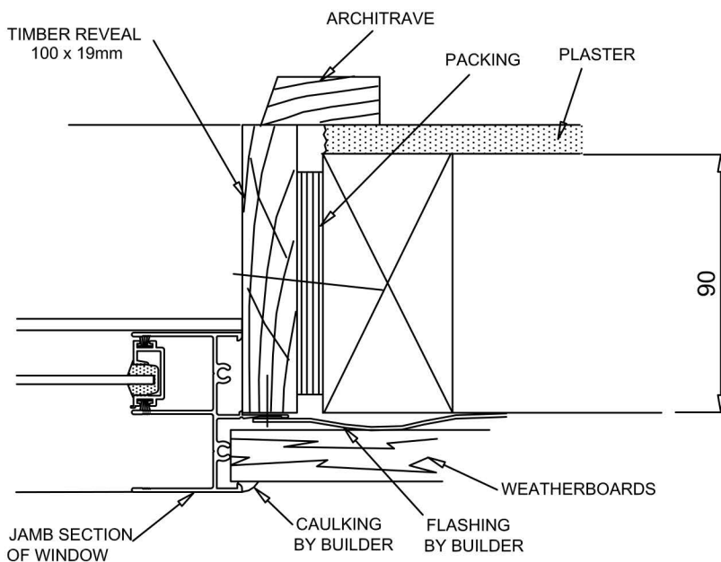
TYPICAL JAMB DETAIL
